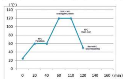
Super transparent clear EVA processing temperature curve graph
