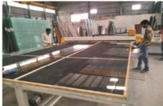
Picture of polishing machine and CNC glass cutting machine imported by the company
