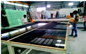
Picture of imported Horizontal Plant and Machinery set-up by the Company
