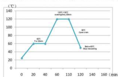
Super transparent clear EVA processing temperature curve graph
