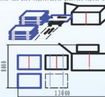
四-七层双工位布局图1 Four and more layers/double position layout diagram
