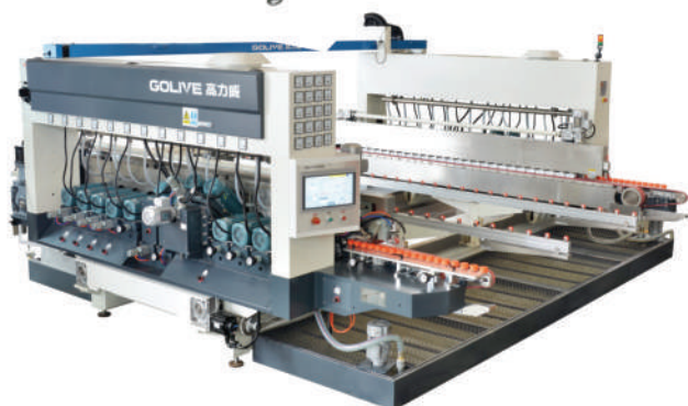
High Speed Glass Double Edger Machine
